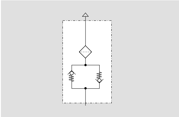
Circuit diagram for ventilating filters with double check valve
