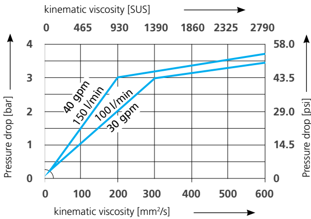
Pressure drop
